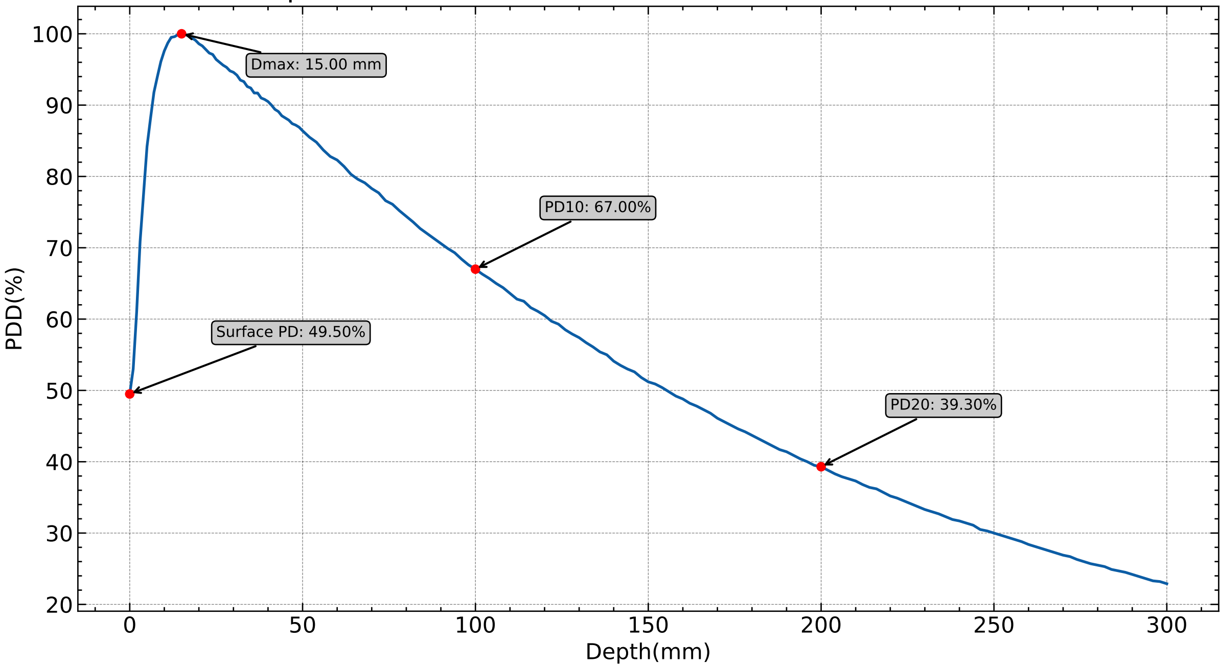
PDD profile of 6MV SSD=100, Water Phantom, F.S= 10x10cm 2
